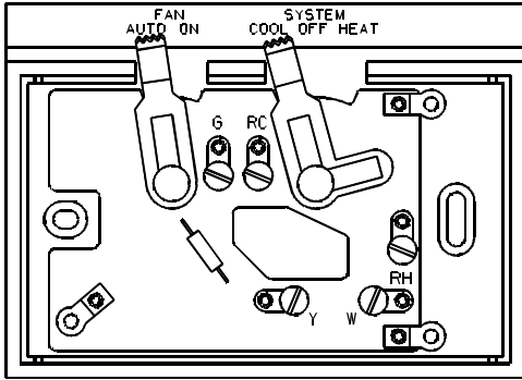
SUB-BASE
