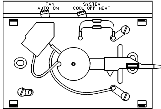
BI-METAL PLATE
